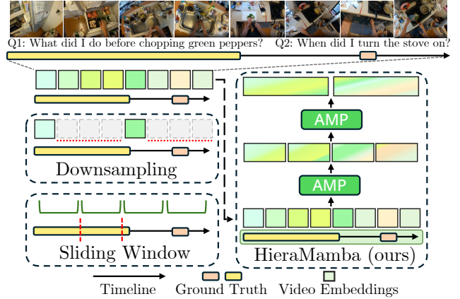
Figure 1. HieraMamba enables hierarchical, linear-time temporal grounding in long untrimmed videos. Top row : a cooking clip and two queries—Q1’s answer spans a long interval, Q2’s a short one. Middle left : uniform downsampling (gray squares) drops frames and loses evidence for the queries. Bottom left : fixed sliding windows split segments at window boundaries but risk fragmenting (red dashed lines). Right : HieraMamba stacks Anchor-MambaPooling (AMP) blocks to build a multi-scale temporal hierarchy that, unlike traditional feature pyramids, uses Mamba to compress and refine information at each level, enabling efficient fine-to-coarse abstraction and precise, query-specific localization. For example, the brief ‘stove on’ moment in Q2 is captured by fine-scale embeddings in the first layer, while Q1’s broader ‘prepping ingredients’ context is naturally represented by the coarser embeddings at the top layer.
